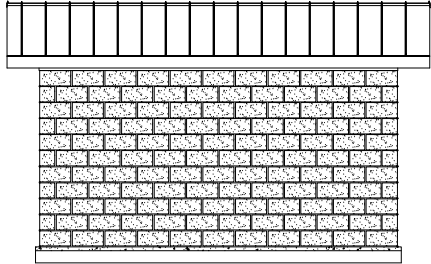
② SIDE ELEVATION 34 GA. DUAL PITCH 1/2" - 1/4" MODEL A
