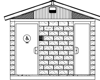
① FRONT ELEVATION 34 GA. DUAL PITCH 1/2" - 1/4" MODEL A
