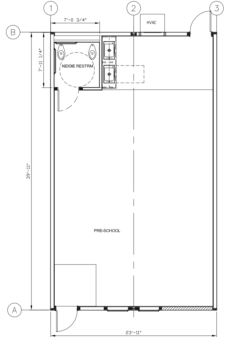
FLOOR PLAN
