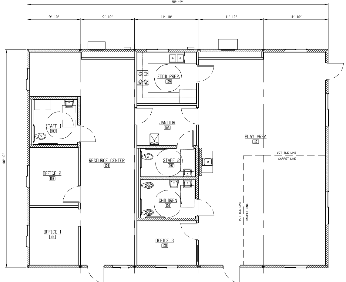
FLOOR PLAN
